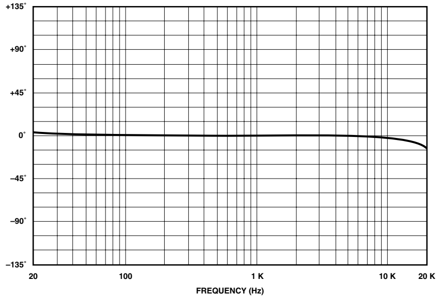
Fig. 6.8 Typical Phase Response
