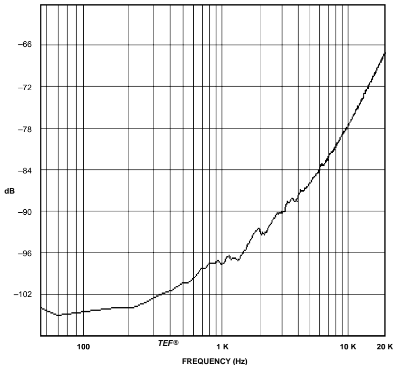
Fig. 6.13 Typical Crosstalk
