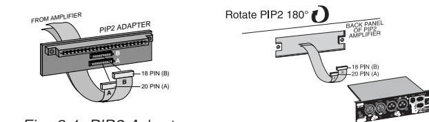
Fig. 8.1 PIP2 Adaptor Connection
