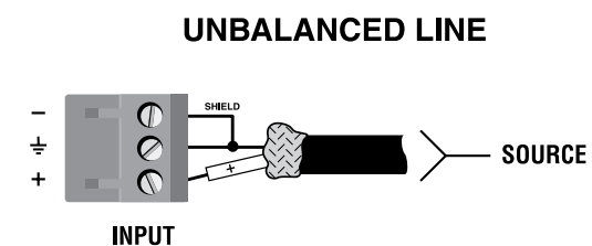
Figure 3.4 Unbalanced Input Connector Wiring
