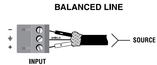
Figure 3.3 Balanced Input Connector Wiring
