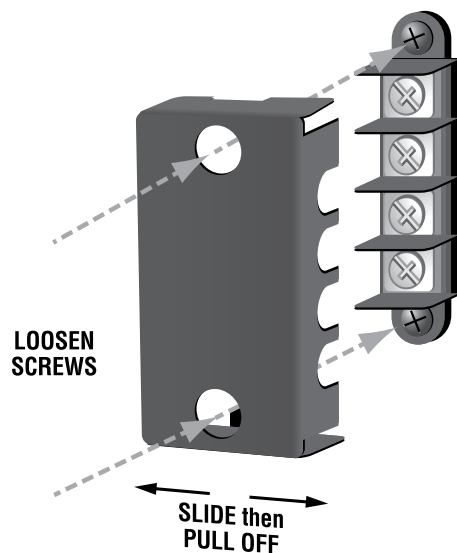
Figure 3.6 How to Remove the Two-Holed Barrier-Block Cover
