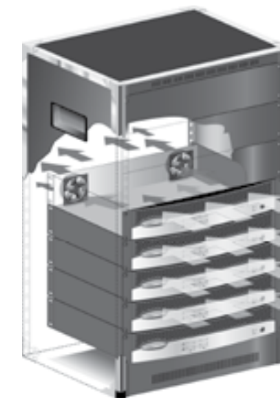
Figure 3.2 Airflow
