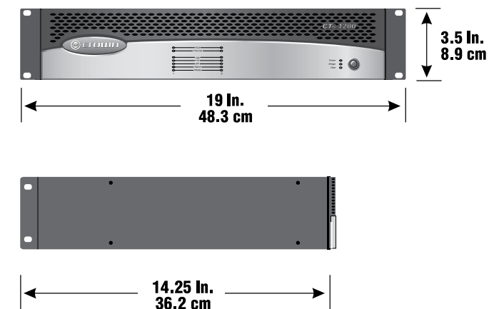
Figure 3.1 CTs 2-Channel Series Dimensions
