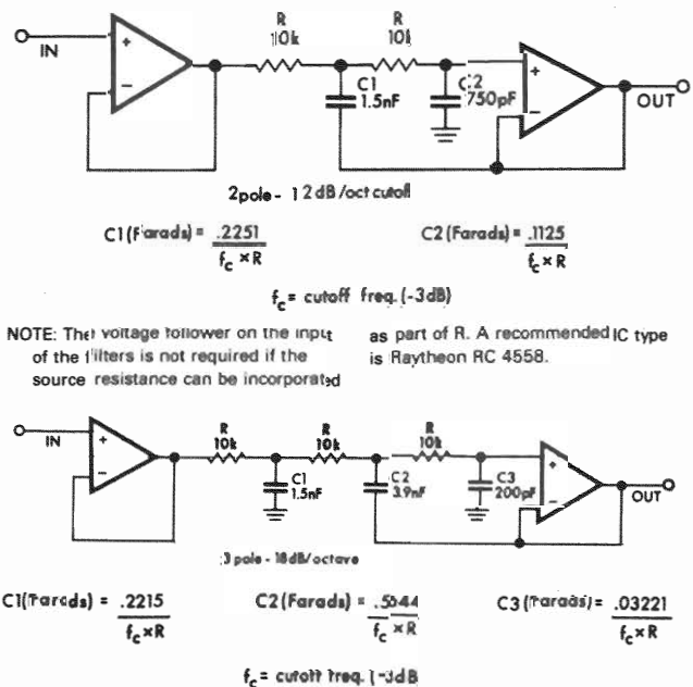
Fig. 3-6. Active L-P Filters
