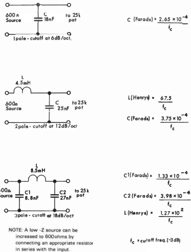
Fig. 3-5. Passive L-P Filters
